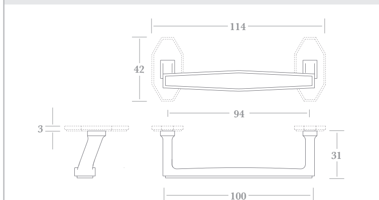
▲ 9504 face fixed
